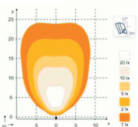
Nordic N4402 LED Wide Flood
