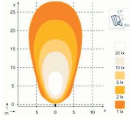
Nordic N4402 LED Flood
